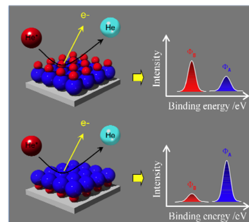
Ultrahigh surface sensitivity of MAES: Outermost electrons are detected!
